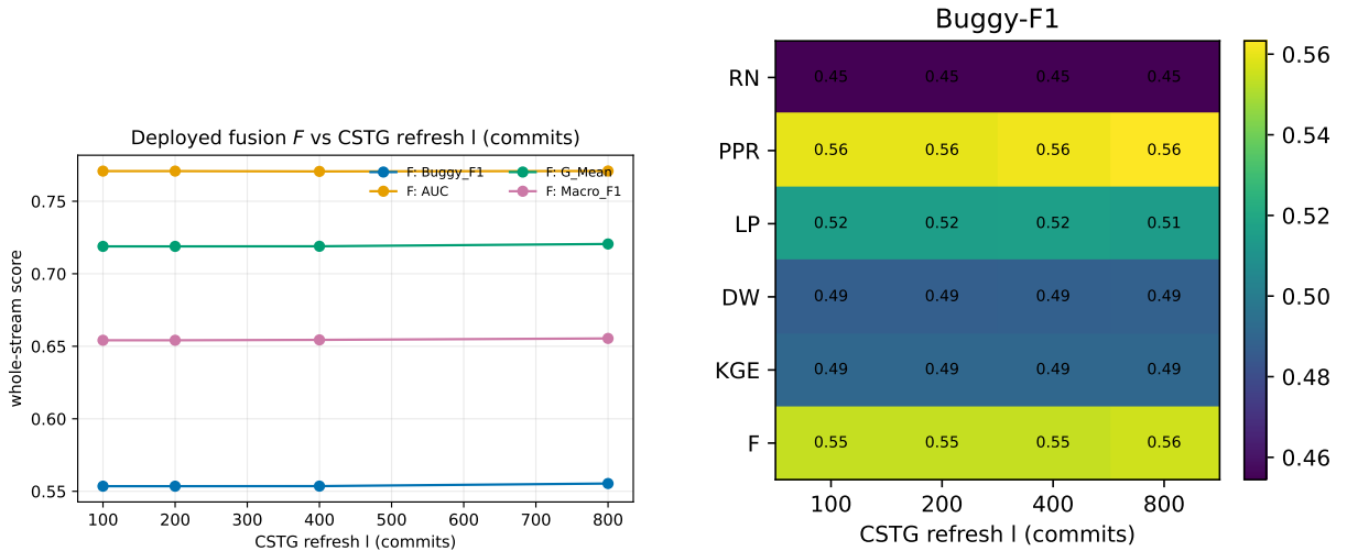
Figure 35: Sensitivity to the online CSTG-hub refresh cadence l : the deployed fusion is essentially flat, so infrequent (cheap) refresh suffices.
