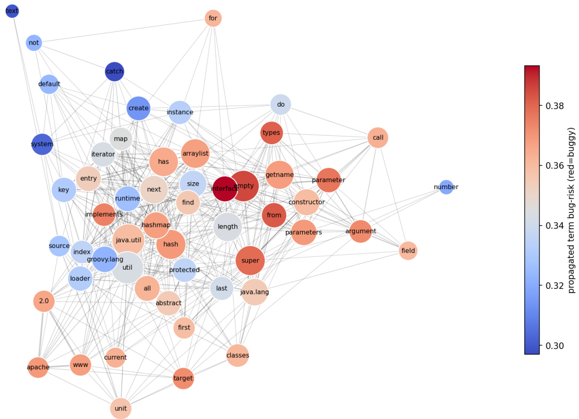
CSTG term co-occurrence graph: NPMI hubs, node colour = propagated bug-risk (semantic communities emerge: buggy type-system/generics terms in red, benign control-flow/instantiation terms in blue)
