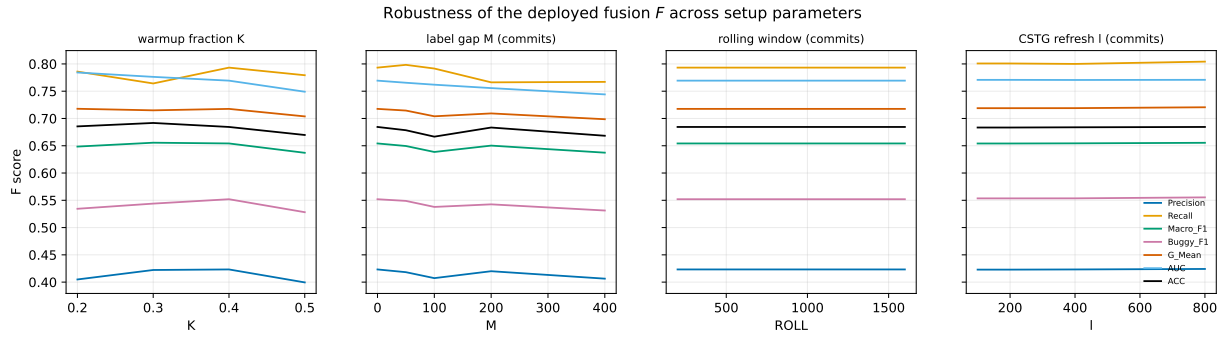
Figure 36: Robustness synthesis: the deployed fusion F 's seven headline metrics against each setup parameter. The model is stable throughout, so the headline conclusions do not depend on the setup.
