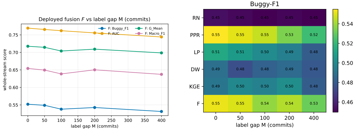
Figure 34: Sensitivity to the label gap M : graceful degradation as recent labels are withheld, with no collapse — the graph structure carries signal even when labels arrive late.
