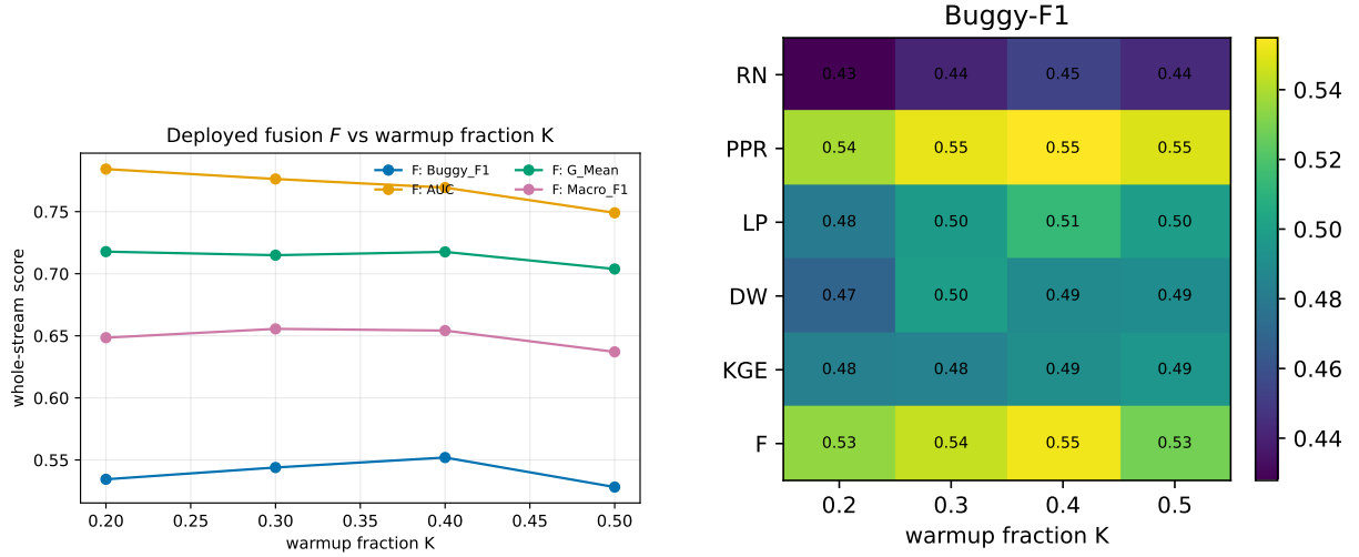
Figure 33: Sensitivity to the warmup fraction K : deployed fusion metrics (left) and Buggy-F1 across methods (right). Near-flat with a mild peak at K \approx 0.4 .
