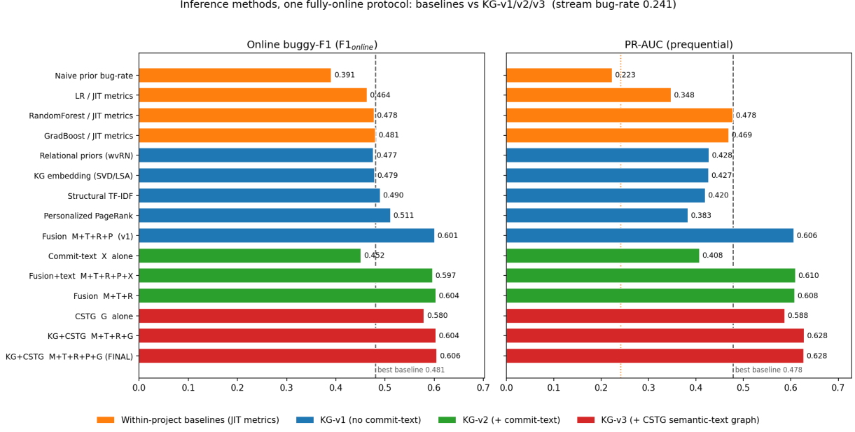
Figure 12: All inference methods under one fully-online (prequential) protocol: within-project baselines (orange), KG-v1 (blue, no text), KG-v2 (green, +commit-text), KG-v3 (red, +CSTG semantic-text graph). Left: online buggy-F1; right: PR-AUC. Dashed line = best JIT-metric baseline.
